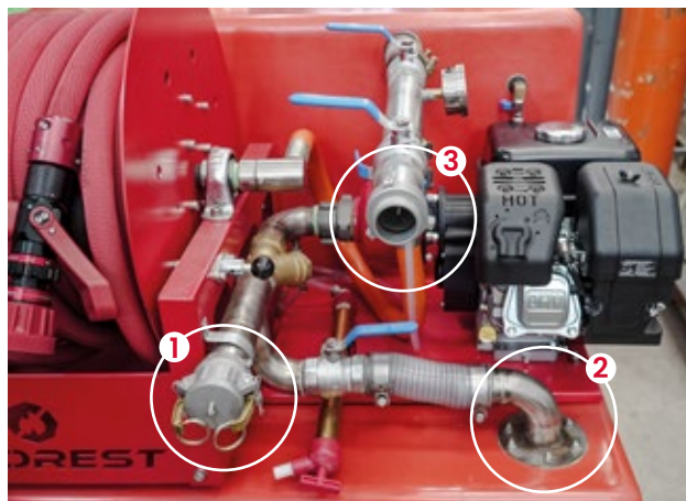
1- Internal suction inlet | 2- External suction inlet 3- Discharge outlet
